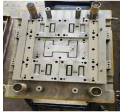
Press Tool Developed for Body of Ammunition Box for Ordnance Factory Bhusawal
